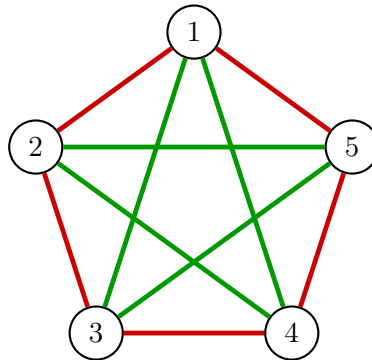
Figure 2: A 2-colouring of K_5 with no monochromatic triangle. Red edges form the outer pentagon; green edges form the inner pentagram. One can verify that no three vertices are mutually connected by edges of the same colour, demonstrating that R(3, 3) > 5 .
